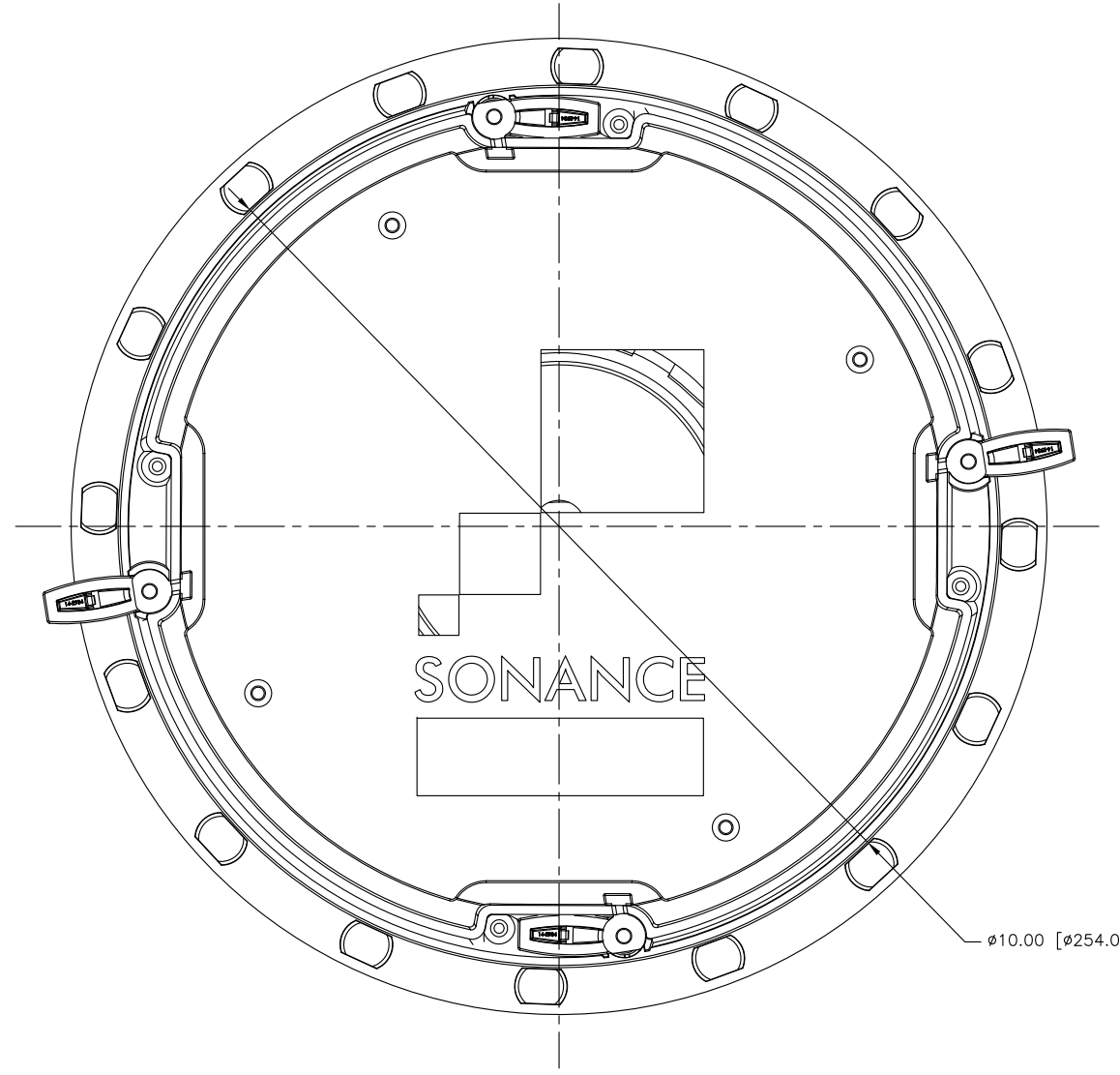
BACK/MINIMUM CUTOUT
